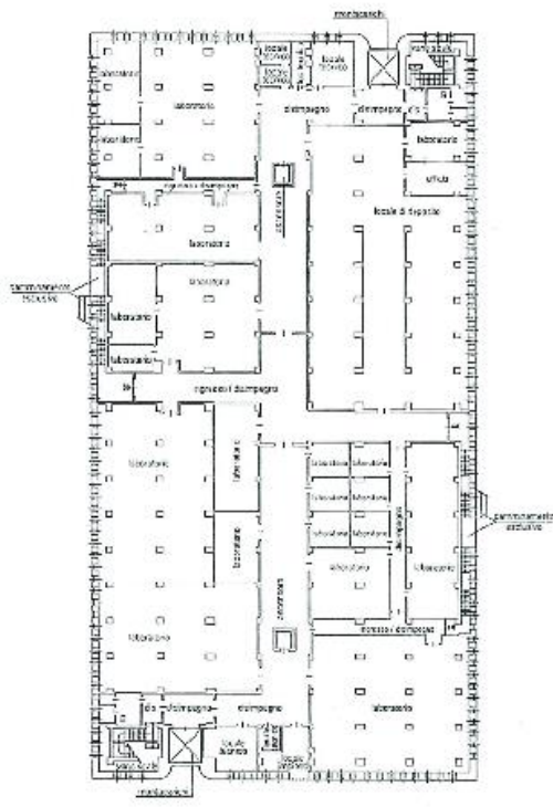
PIANO INTERRATO h 4.10 m
